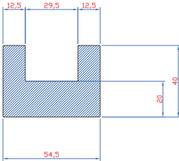
Small U Channel (For Bottom)
