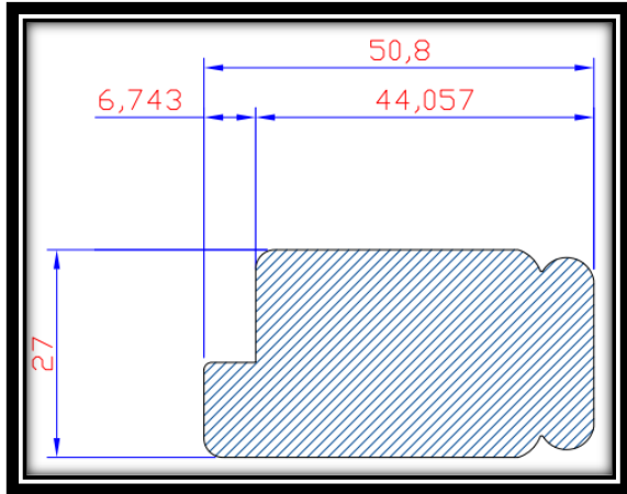
Beaded Stile (Default)
