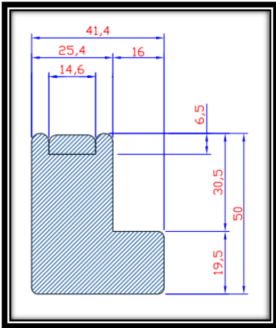
Small Face Fit L Frame
