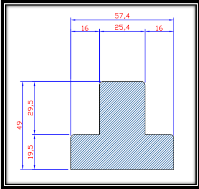
T Post
