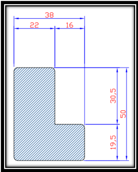
Small L Frame Flat
