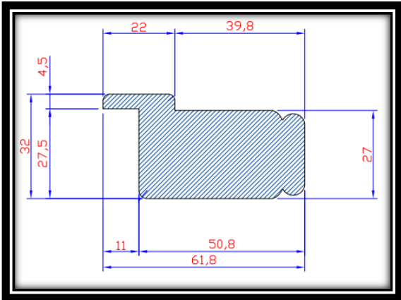
D-Mould Stile (Beaded)
