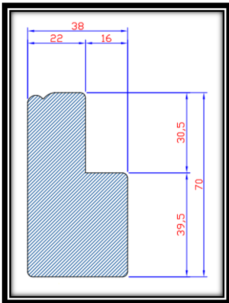
Medium/Large L Frame (Beaded Option)
