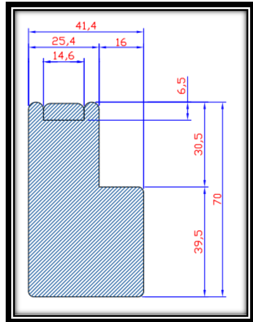
Medium / Large Face Fit L Frame
