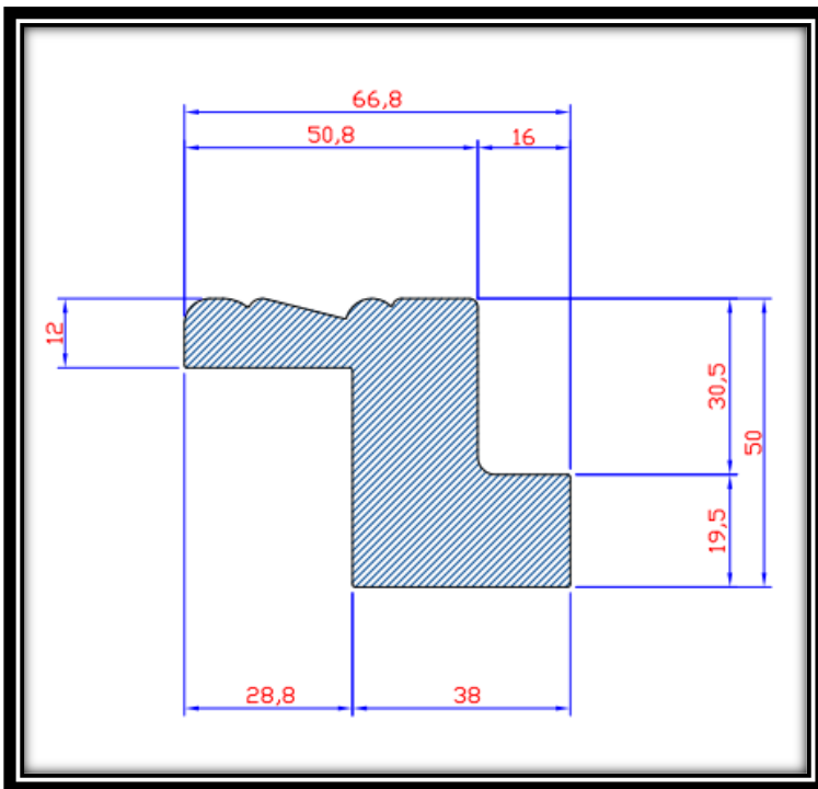
Standard Z Frame
