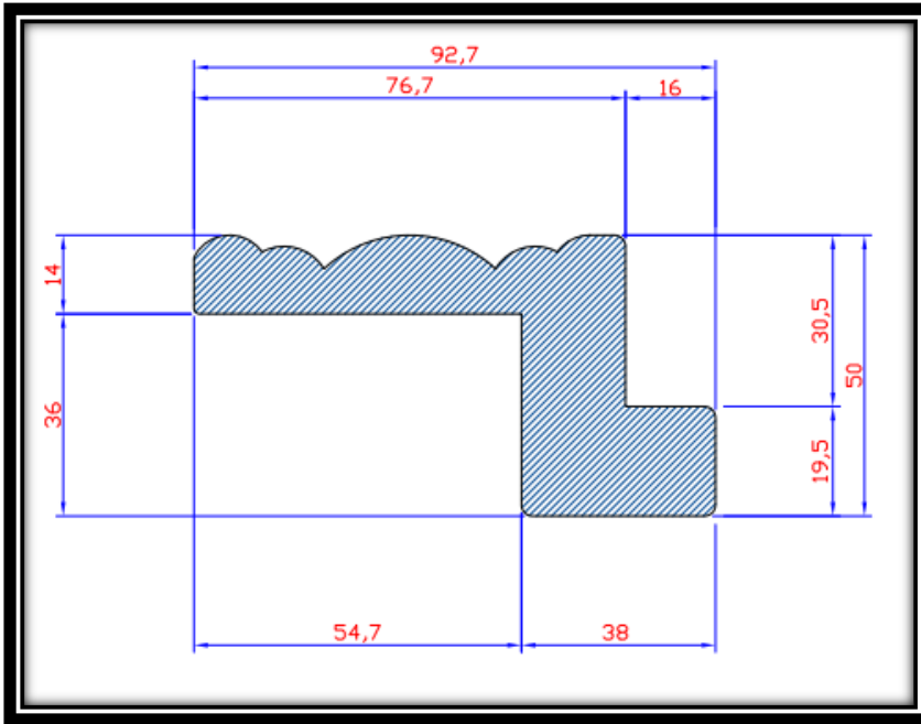
Large Z Frame
