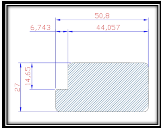
Flat Stile (Optional)
