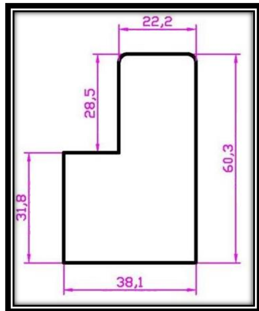
Medium L Frame Flat
