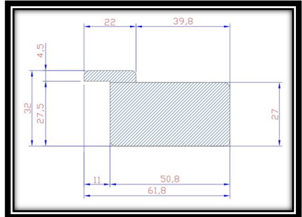
D-Mould Stile (Flat)
