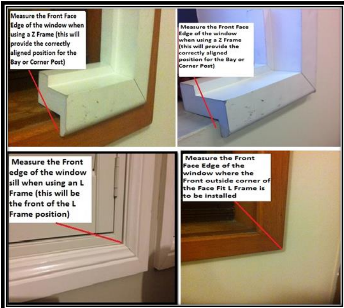
Examples of Frame Position
