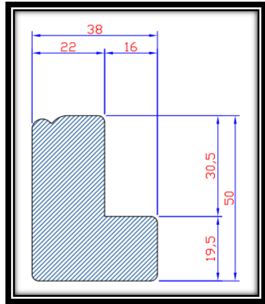
Small L Frame (Beaded Option)
