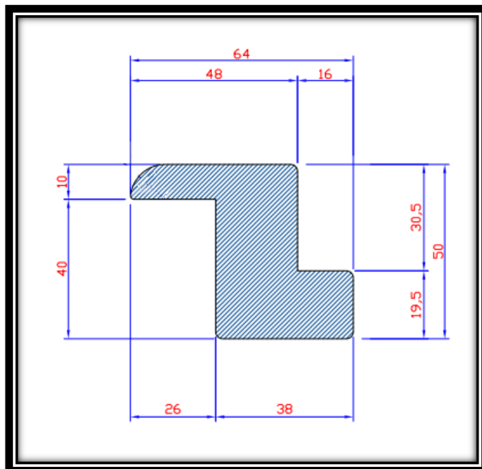
Large Bullnose Z Frame
